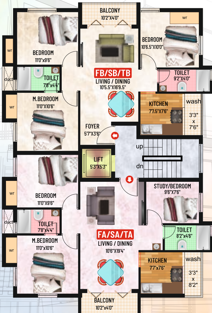
SITE CUM TYPICAL FLOOR PLAN [ I , II & III ]
